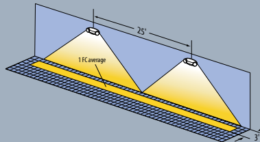
example of multiple ELM2 LED unit illuminating a 3" path of egress
