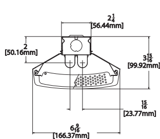
Two-lamp T5
