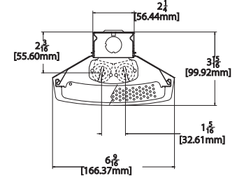
Two-lamp T8
