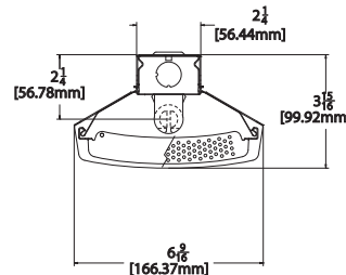
One-lamp T8
