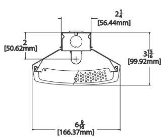
One-lamp T5
