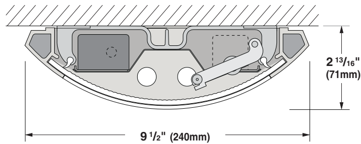
SUR9-2T5 Surface Mount
