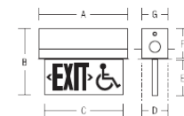
Recessed Wall
