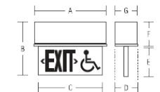
Surface Wall
