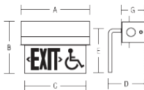
Recessed Wall
